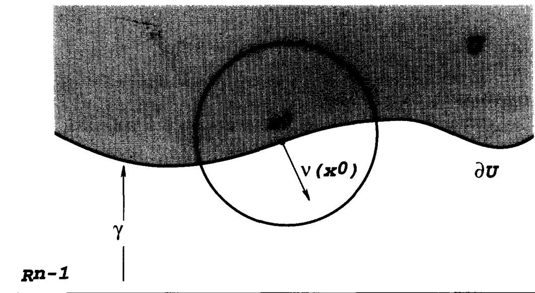
The boundary of U
