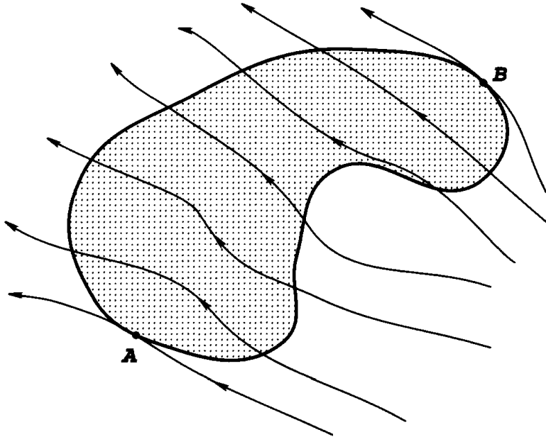
Case 1: flow to an attracting point
