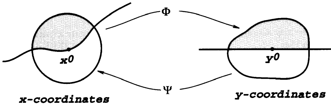
Straightening out the boundary
