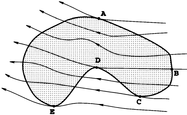
Case 3: flow with characteristic points
