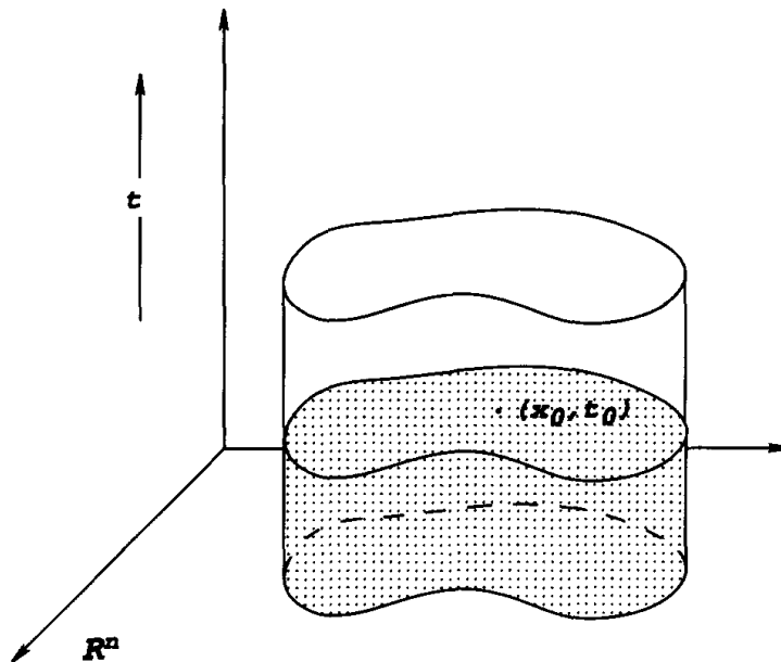
Parabolic strong maximum principle
