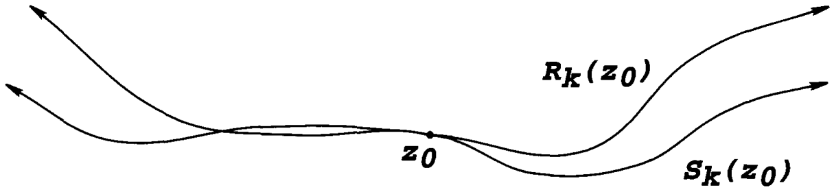
Contact between R_k and S_k
