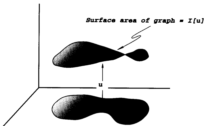
A minimal surface
