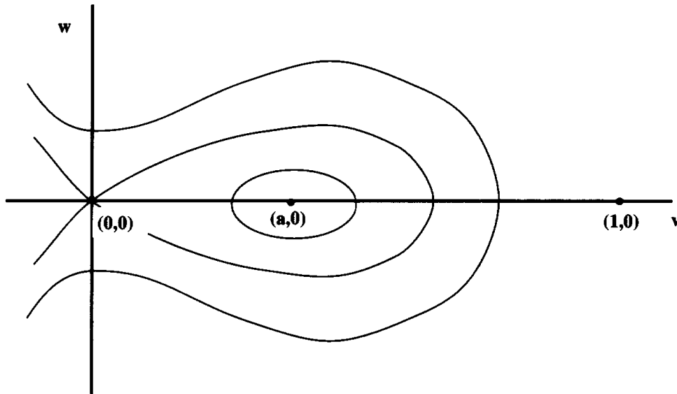
Level curves of E
