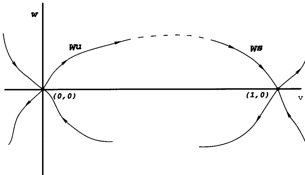
Stable and unstable curves
