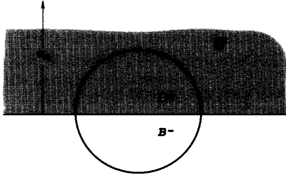
A half-ball at the boundary
