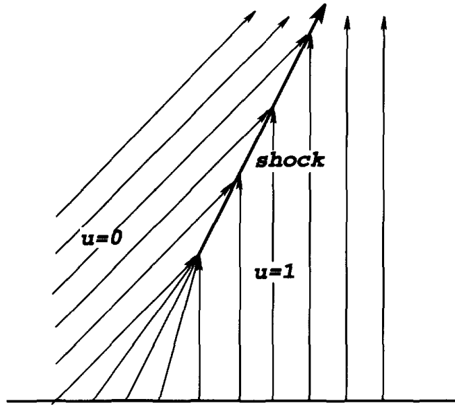
Formation of a shock
