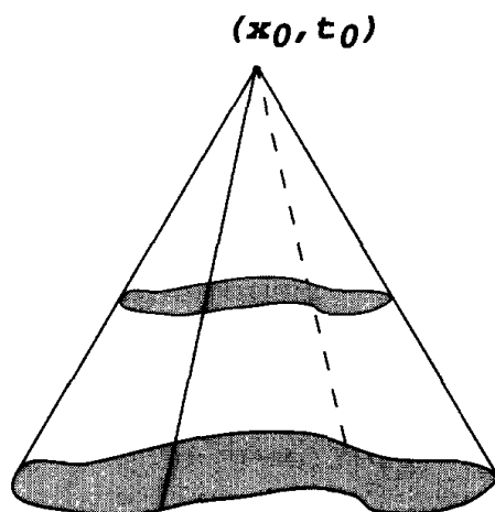
Domain of dependence
