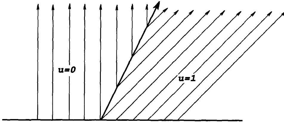
A "nonphysical" shock
