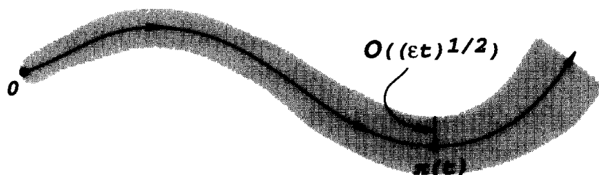
Flow of dye with diffusion
