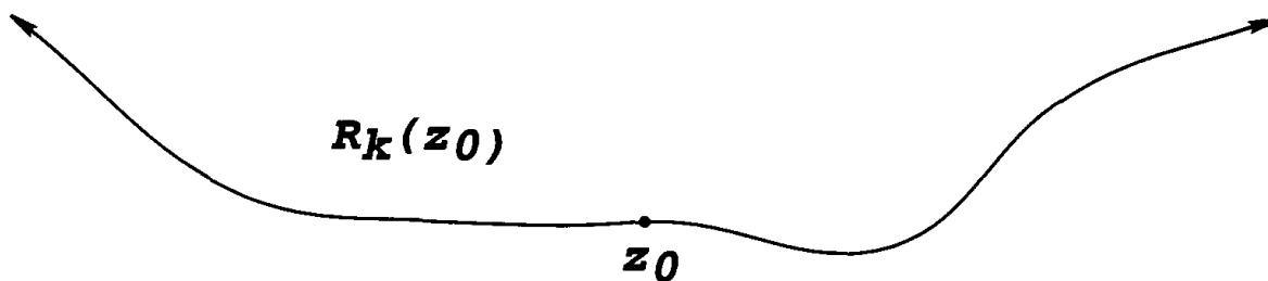
Rarefaction curve
