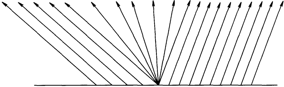
k -rarefaction wave
